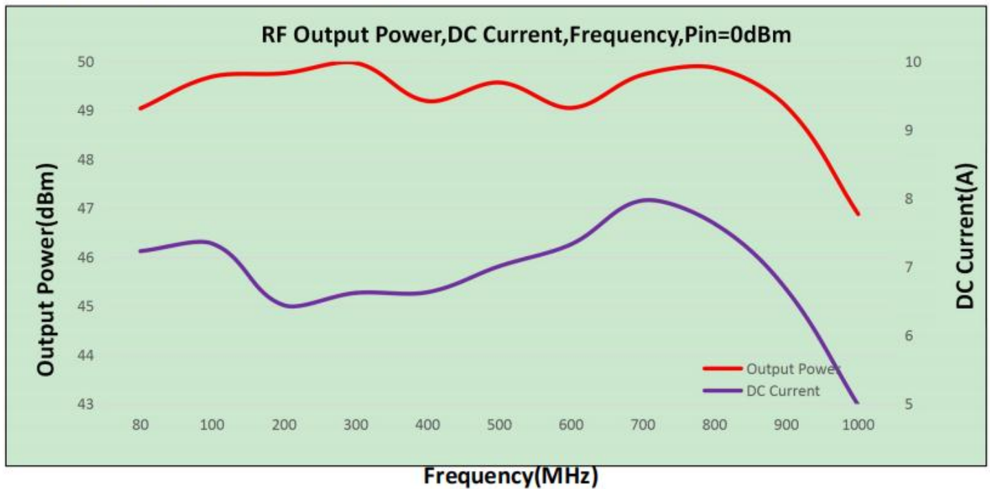
Graph 3: RF Output Power (Normal temp. +25\pm 3^{\circ}\text{C} )
